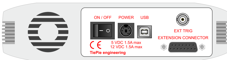
Figure 7.1: Rear panel
