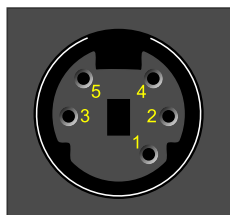
Figure 7.2: Power connector
