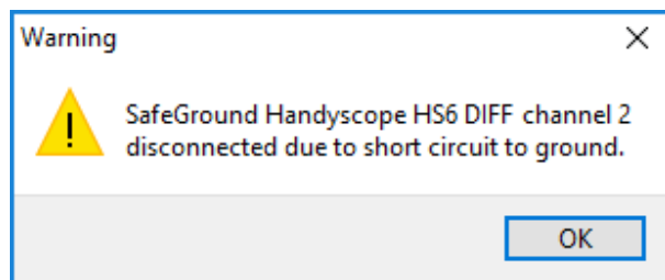
Figure 4.4: SafeGround warning
